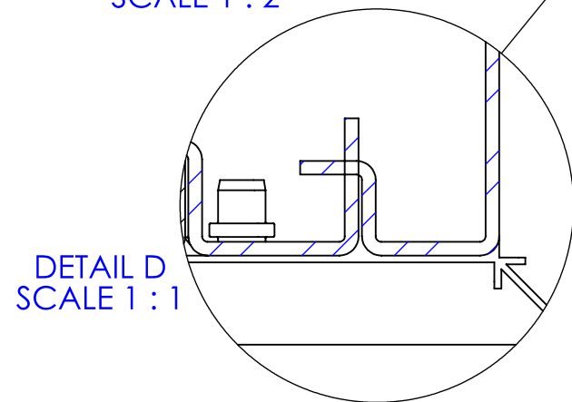
Ground pin
