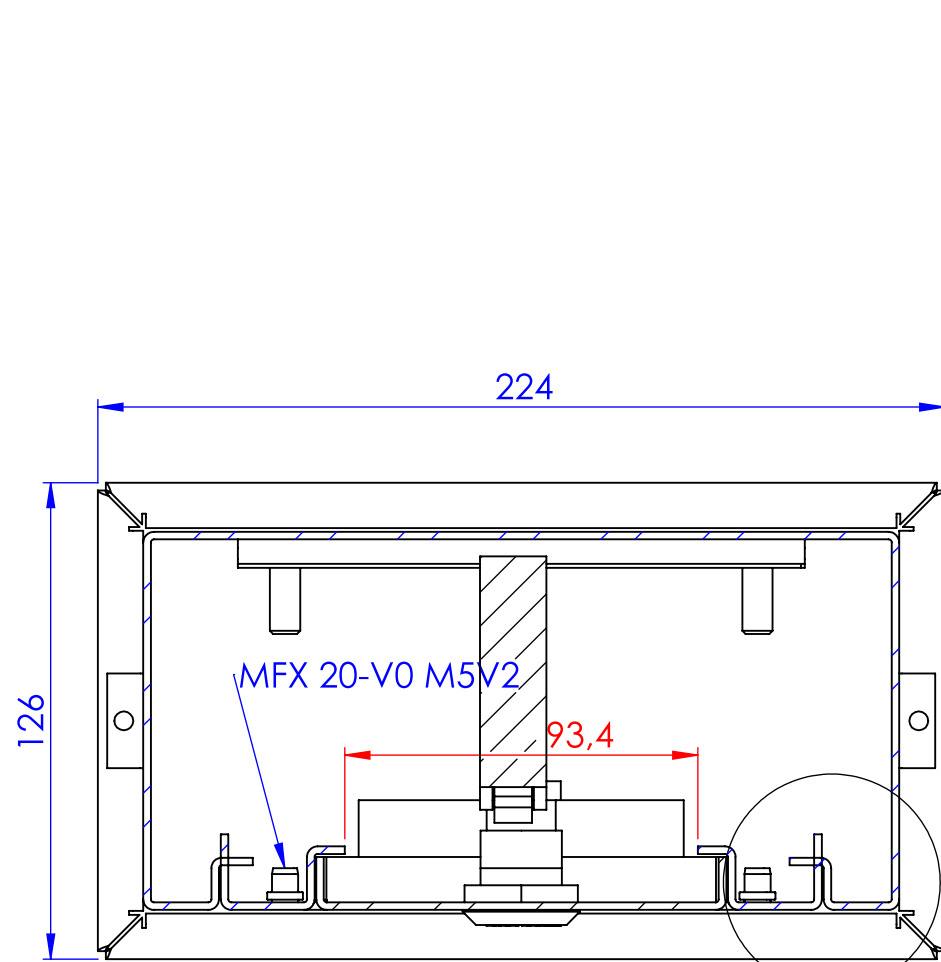
SECTION C-C SCALE 1 : 2
