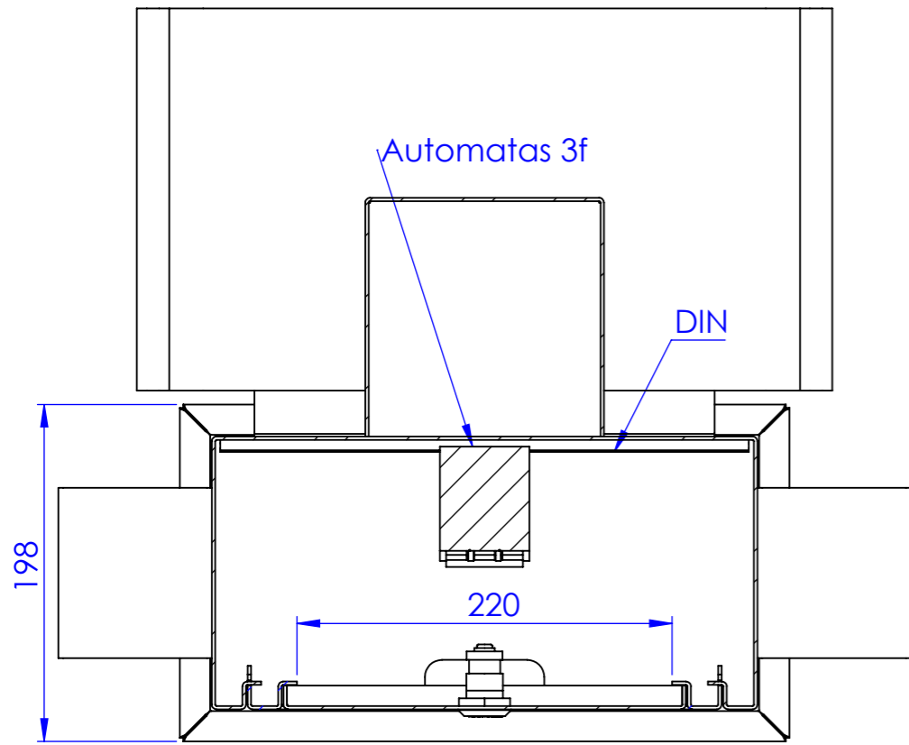
SECTION C-C SCALE 1 : 4
